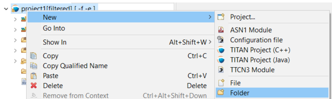
Figure 32. New menu
