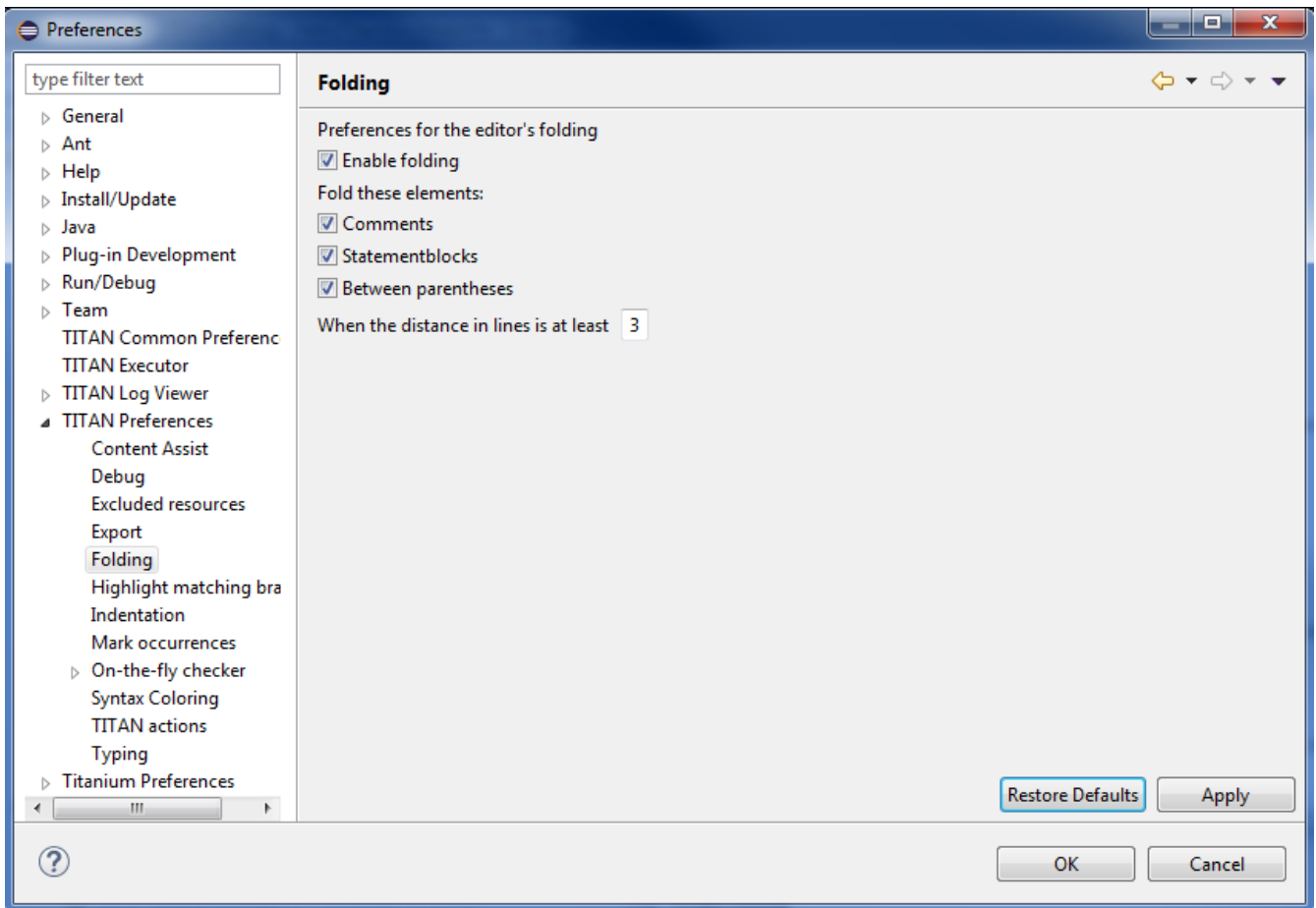
Figure 20. Folding preferences
