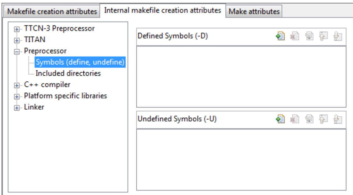
Figure 46. Preprocessor symbols
